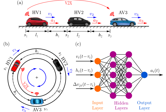
Fig. 1. (a) Virtual Ring setup: The automated vehicle AV3 drives in front of two human driven vehicles, while it receives the position and velocity of the last HV via V2X communication. The control of AV3 is designed in a way as if HV1 was in front of it. (b) The corresponding ring configuration. (c) Time delay neural network with two hidden layers, which was applied to learn the human driving dynamics.
